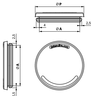
Double parallel membrane
